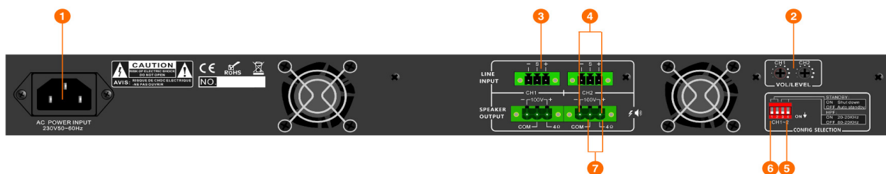
Figure 2: BA Series Rear View
