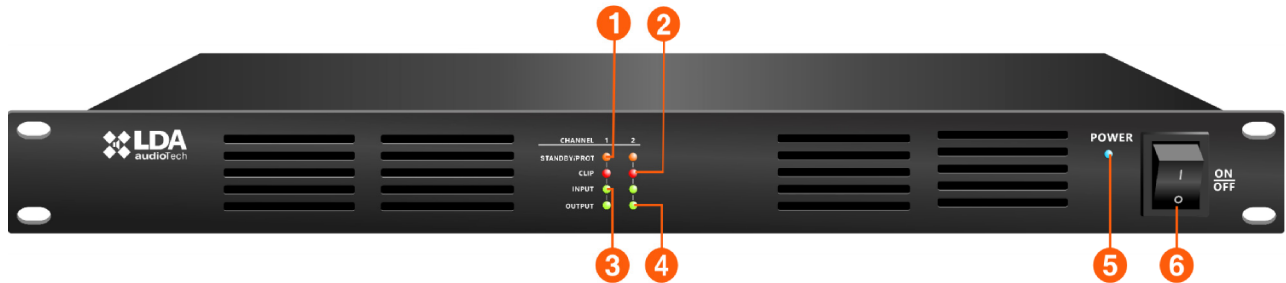
Figure 1: BA Series Front View
